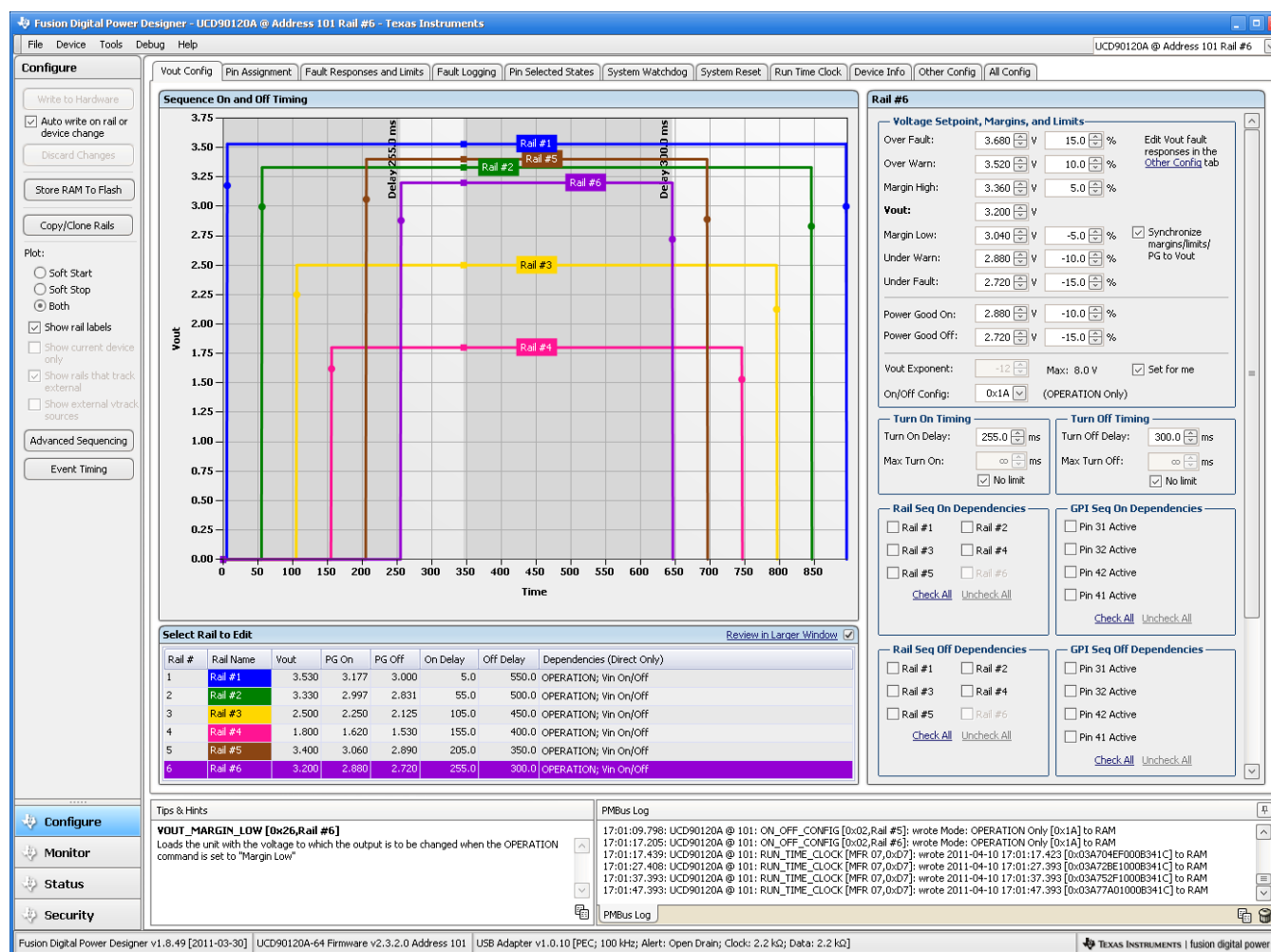
Figure 7. Fusion GUI V OUT -Config Tab
