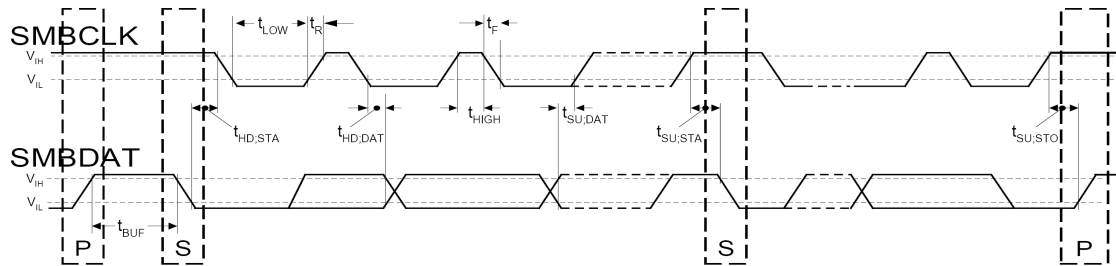
Figure 1. I²C/SMBus Timing Diagram
