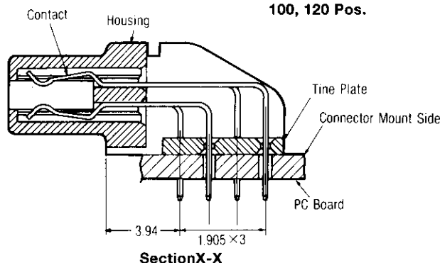
Section X-X
