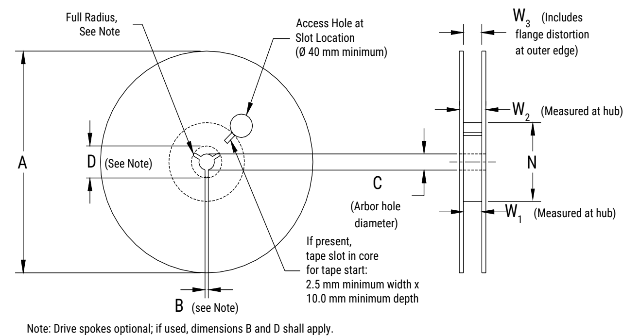
Figure 5 – Reel Dimensions
