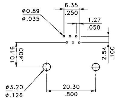
PCB LAYOUT
