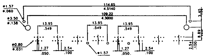
PCB LAYOUT 8 PORTS
