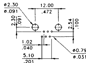
PCB LAYOUT C026-6
