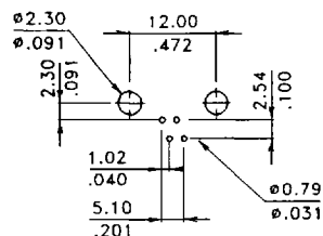
PCB LAYOUT C026-5
