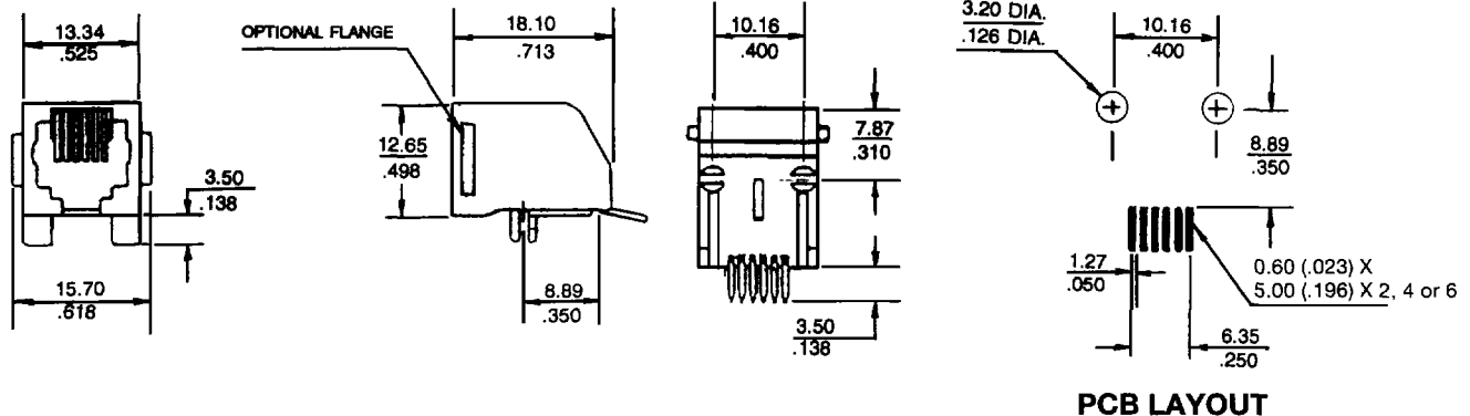
PCB LAYOUT
