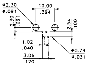
PCB LAYOUT C026-4
