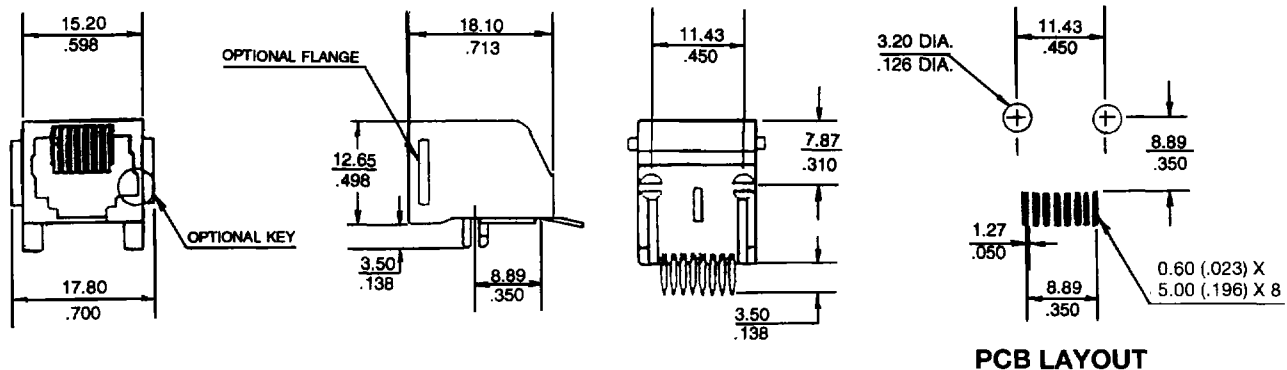
PCB LAYOUT
