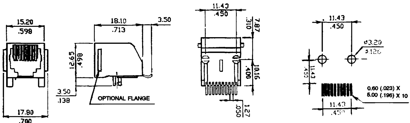
PCB LAYOUT
