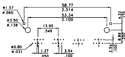
PCB LAYOUT 4 PORTS
