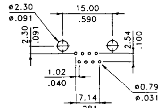
PCB LAYOUT C026-7 C026-8
